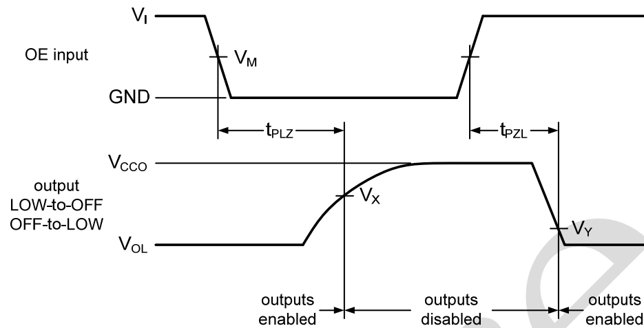
Figure 3. Enable and disable times
