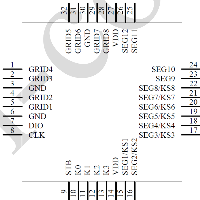
LQFP32
