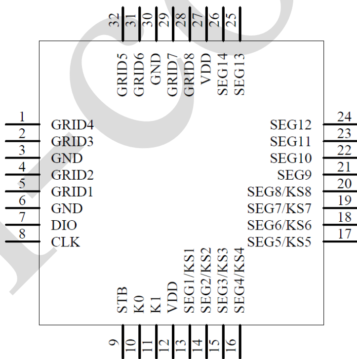
LQFP32
