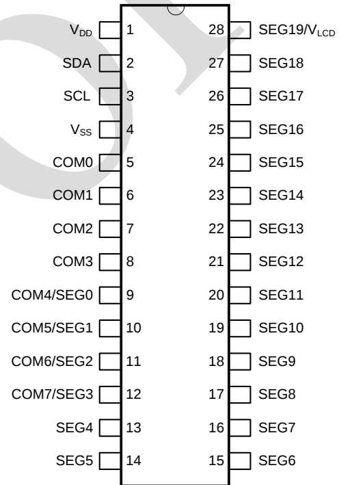
SOP28/SSOP28
