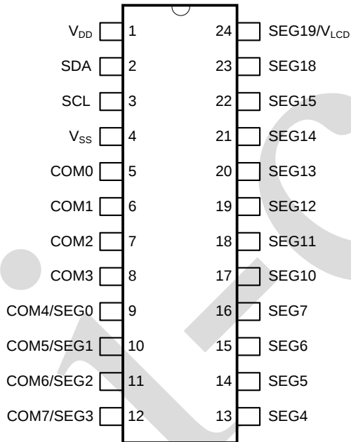
SOP24/SSOP24
