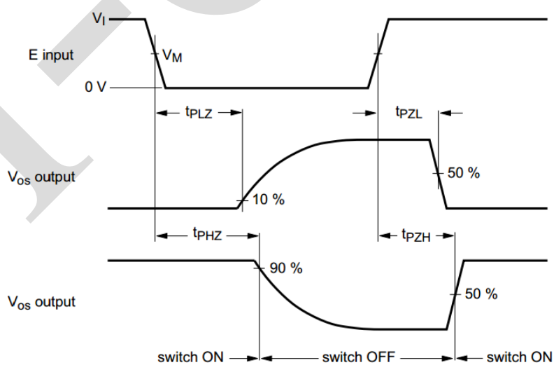
Figure 9. Turn-on and turn-off times
