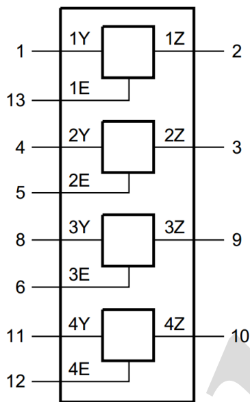
Figure 1. Logic symbol
