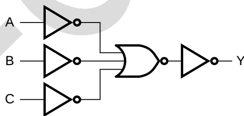
Figure 3. Logic diagram for one gate
